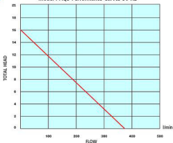
Model : AQ3 Performance Curves 50 Hz
